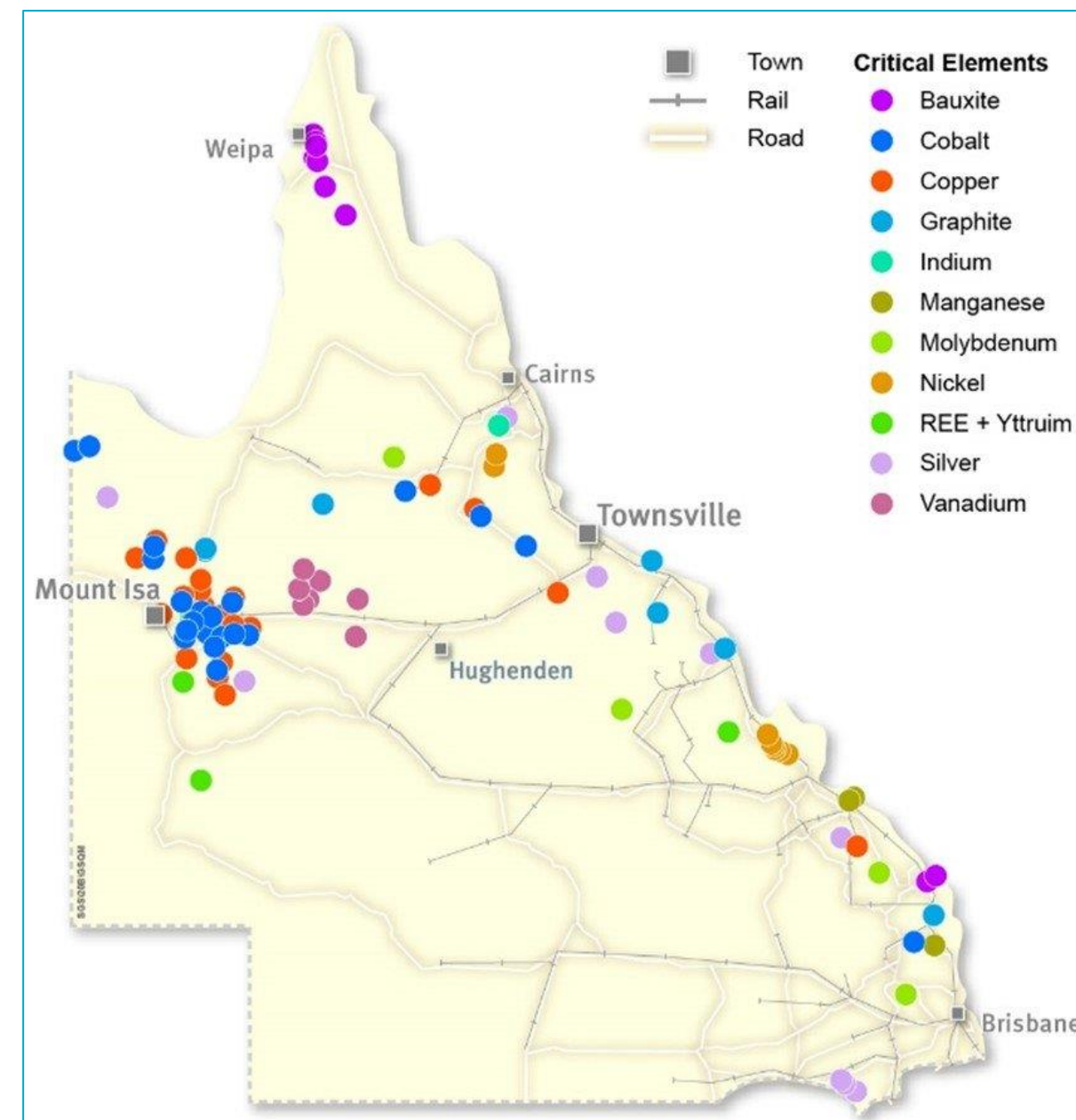
An overview of Queensland new economy mineral deposits. Source: AusIMM Bulletin Sept 2020: 'Queensland's New Economy Minerals Initiative', Helen Degeling
